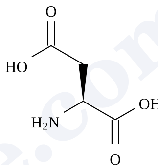
Aspartic acid
